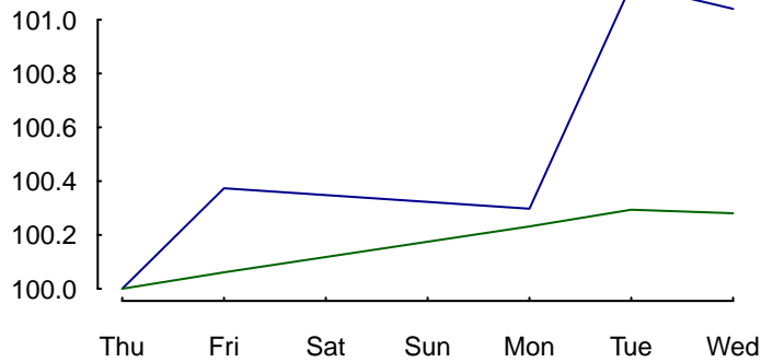
Figure 8.1: Scaled series: Both dax and rexp now start at 100.
